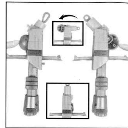
5) Rotate head into slot until blade is straight up.
